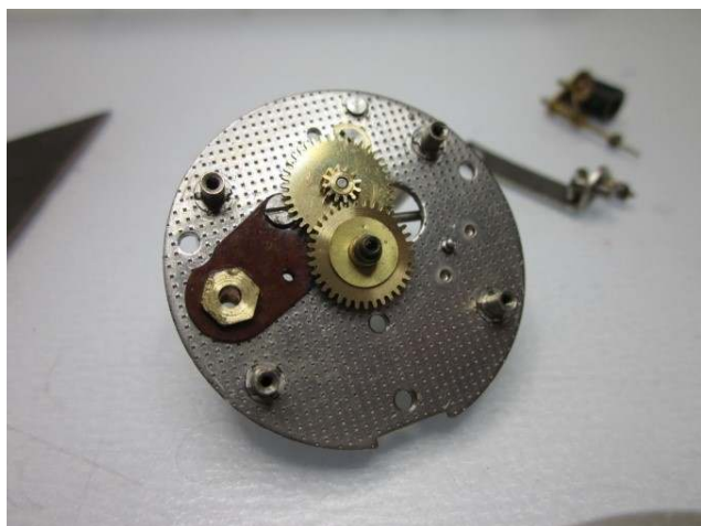
Photo 5 - Front of the clock with hands and dial removed.
